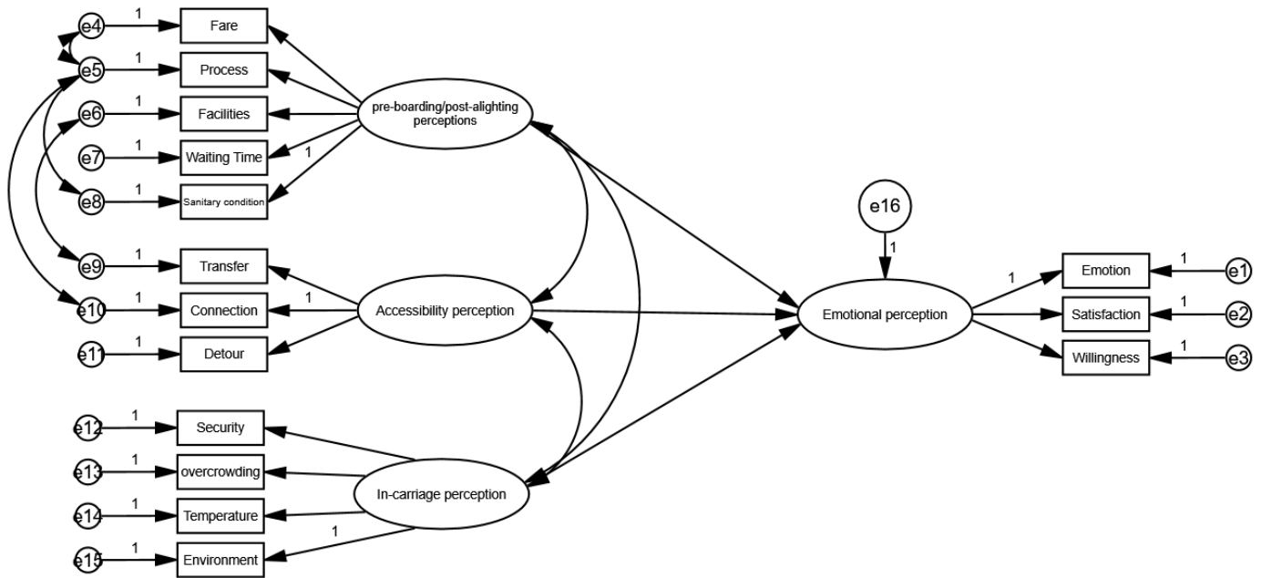
Figure 3 | Path Diagram of the SEM Model
