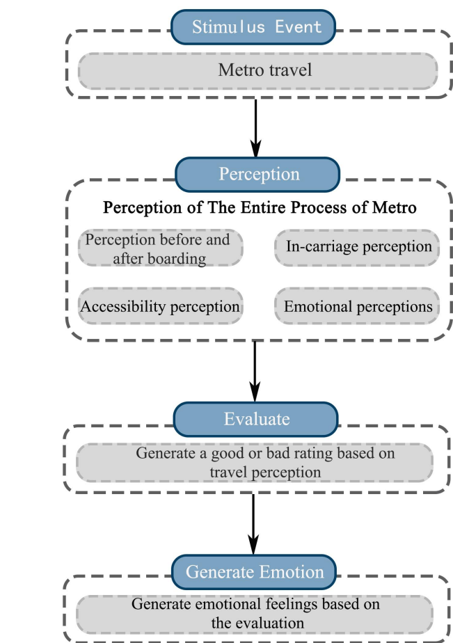
Figure 1 | Path Diagram of Metro Travel Emotion Generation
