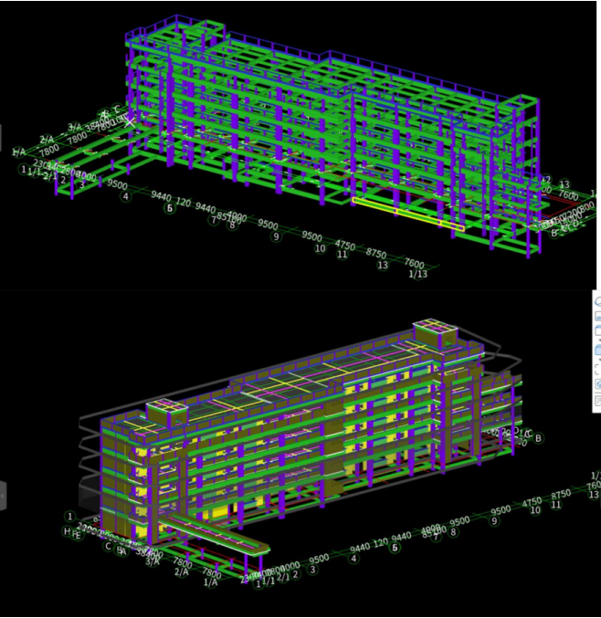
Figure 2 | Architectural appearance (BIM diagram in Glodon GTJ2021)
