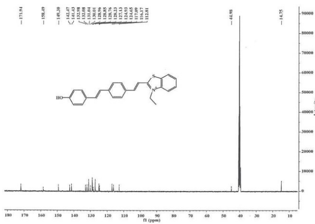
Figure 20 | Carbon spectrum of HO-PPV-EtBT
