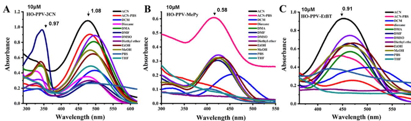
Figure 7 | Uv-vis absorption spectra of fluorescent dyes HO-PPV-3CN, HO-PPV-MePy and HO-PPV-EtBT (Concentration=10 \mu m) in different solvents at 25°C, slit width: 10/10 nm.
